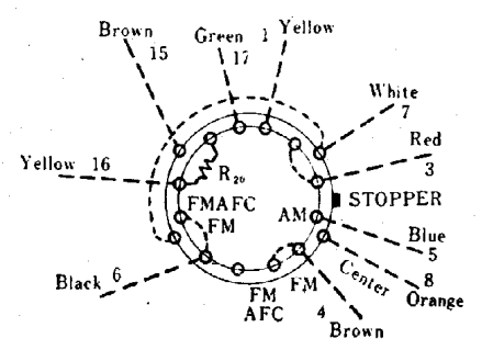
Band setting switch (Bottom view)
